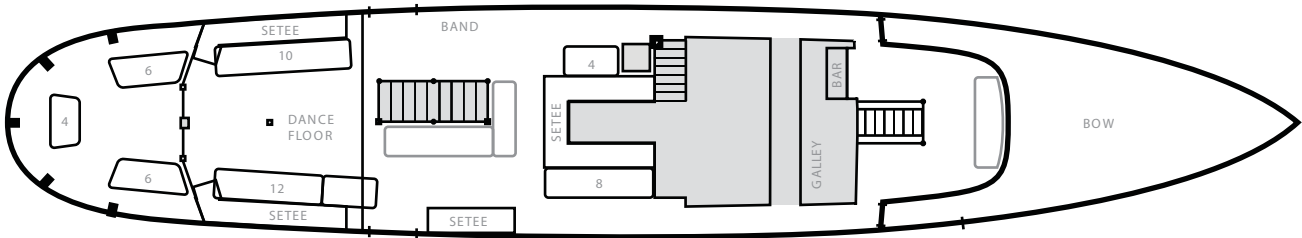
MAIN DECK
